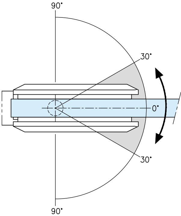
automatic closing action from 30^\circ "Zero point" ( 0^\circ - closing) adjustable
